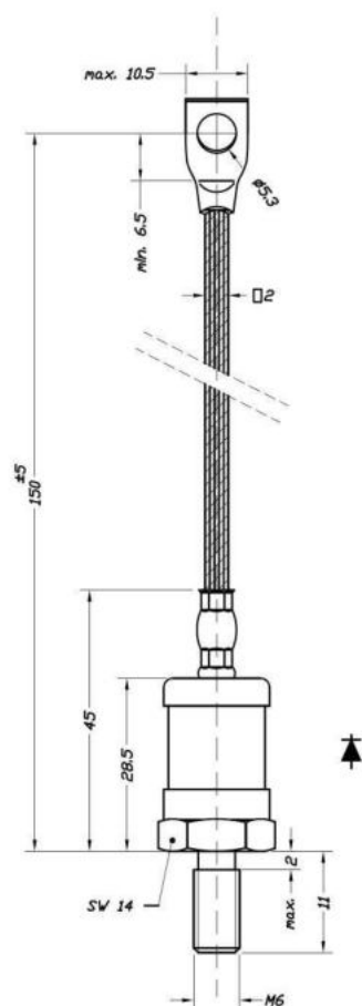
CASE E 42 (IEC 60191: A 16 M modified)
